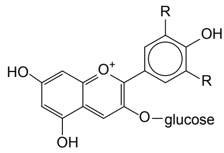
flavylium cation (red)
